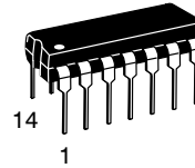
PDI-14 N SUFFIX CASE 646
